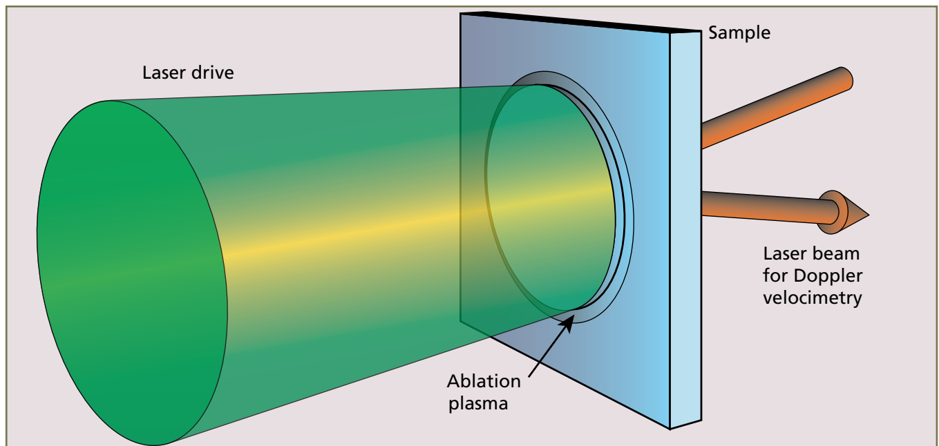
Schematic of laser ablation experiment on material response. The laser pulse creates a region of plasma, driving a shock wave into the sample. Motion of the opposite surface is monitored by Doppler velocimetry using a second laser.
