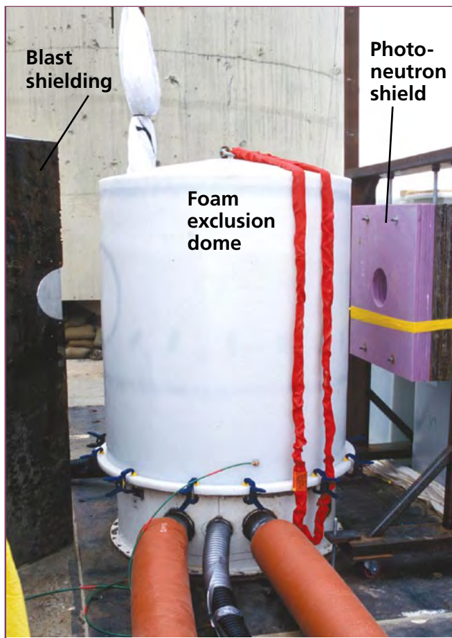
Foam exclusion dome. To avoid exposing test components to the containment foam, DX personnel sealed all 3612 and 3625 components in a container similar to this one used for shot 3605. Red strapping cables were used to emplace the dome; the two red cables at bottom protected pin harnesses from the containment foam after emplacement.
