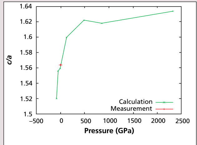
Calculated variation of c/a ratio with pressure, and value measured at STP.
