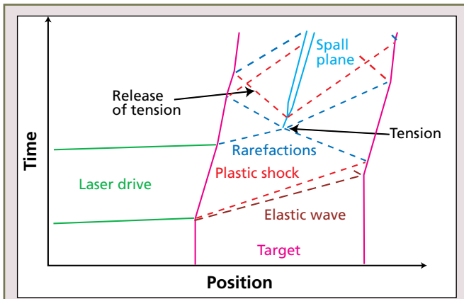
Position-time diagram of waves induced by laser ablation. Note the elastic precursor running ahead of the initial plastic shock. Information on the flow stress can be derived from the velocity history of the surface as the elastic and plastic waves appear.
