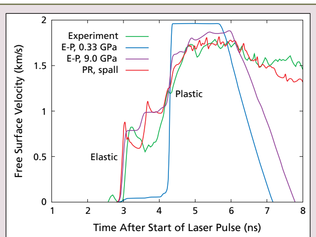
Velocity history from the free surface of a beryllium crystal, compared with simulations using different models of plasticity. Elastic-plastic (E-P) simulations are the simplest models of plasticity; 0.33 GPa is a typical flow stress on microsecond time scales. The elastic wave breaks out at the correct time, but the amplitude is too low and the shape of the plastic wave is incorrect. Increasing the flow stress to 9 GPa improves the amplitude but not the shape. The plastic relaxation (PR) model reproduces the shape of the elastic wave more accurately; this model did not include work hardening, so the rising part of the elastic wave shows stronger reverberations in the simulation than we observed experimentally. The PR simulation also included spall, improving the match after the peak of the plastic wave. Note that more accurate simulations of the elastic wave also improve the match in the plastic region.
