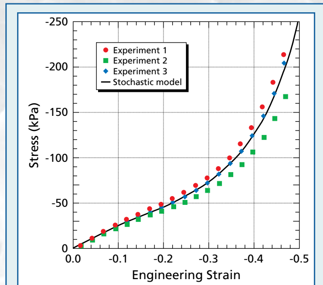
Continuum-scale, stress-strain response. Three silicone foam samples were subjected to uniaxial compression. Each sample was a highly disordered, open-cell silicone foam with identical average material properties. LANL scientists used a stochastic constitutive model to simulate the response of this material to quasi-static loading conditions. For the uniaxial deformations considered here, engineering strain is directly related to the ratio of compression (i.e., the length of the compressed specimen divided by the original length).
