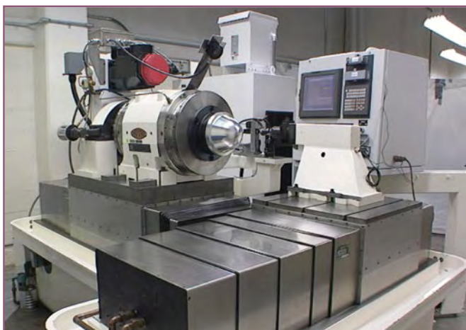
Moore T-base lathe with unclassified part. The retrofit of a Moore T-base lathe completes the first phase of a collaborative project that reduced security risks by eliminating classified computer disks and shortened in-process inspections from hours to minutes.
