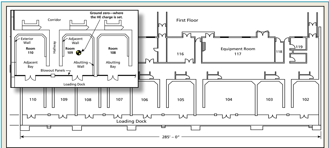
This diagram shows the layout of building 340 and its nine bays (rooms 102–110). The inset shows an adjacent bay and an abutting bay.
