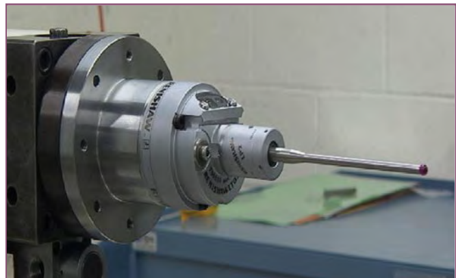
Renishaw LP2 probe. Using standard off-the-shelf hardware, MSM engineers and machinists designed software that measures components during the machining process, eliminating the need for manual part removal, inspection, and reinstallation. Using on-machine probing reduces the risk of handling errors that result in damage to component parts.
