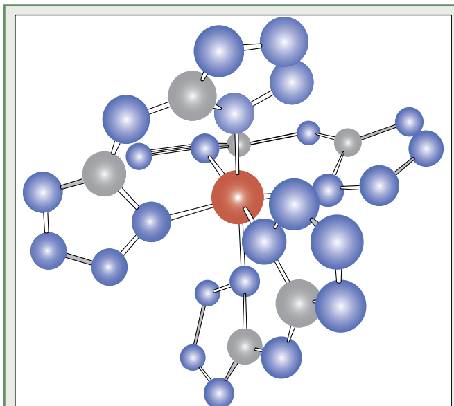
The (\text{NH}_4)_3[\text{Fe}^{\text{III}}(\text{BTA})_3] anion of iron-bistetrazolamine (Fe-BTA). This anion is the high-nitrogen transition-metal complex we use to produce iron nanofoam. This was the first material we investigated to produce metal foams. The blue spheres are nitrogen atoms, the gray spheres are carbon atoms, and the red sphere is an iron atom. We replace the iron atom with an atom of a different metal to produce a complex of a different metal. Not shown are the three ammonium cations surrounding the anion.
