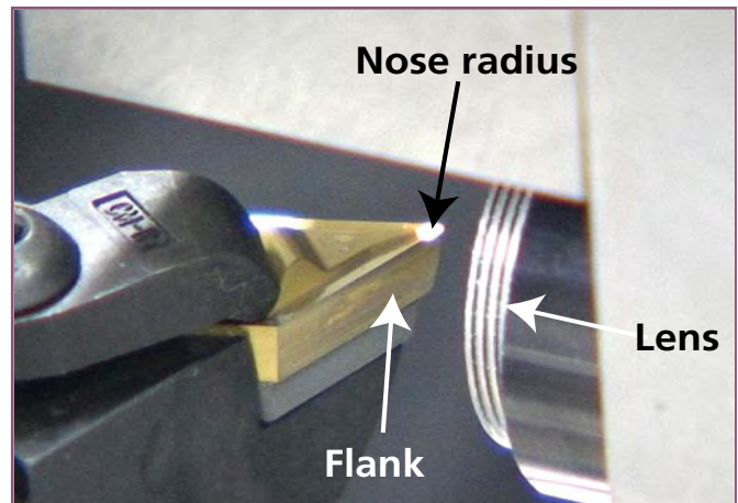
Cutting-tool insert. The numerous advantages of using industry-developed cutting tools (inserts) to fabricate nonnuclear weapon components include reduced cost, extended tool life, better chip control, less machining time, less waste stream, and improved surface finishing.
