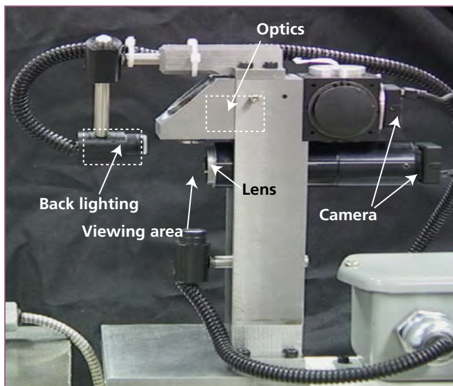
Optical tool locator. MSM machinists and engineers devised a multifunctional tool locator that characterizes and orients the cutting insert during fabrication. Imaging the tool in two views, the locator correctly positions the insert and automatically updates the lathe's cutting-tool registers.
