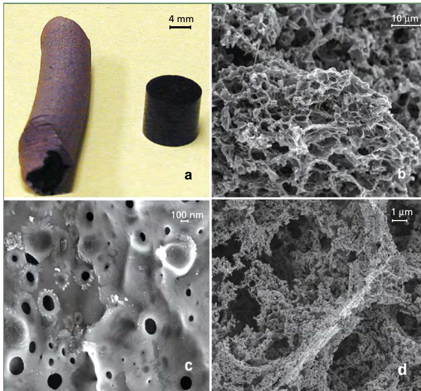
Iron pellet and examples of iron nanofoam: (a) photograph, 4-mm scale bar, of iron foam monolith next to unburned pellet of the Fe-BTA complex; (b) SEM, 10- \mu\text{m} scale bar, of low-pressure iron foam showing pore structure of roughly 1 \mu\text{m} ; (c) SEM, 100-nm scale bar, of high-pressure iron foam showing pore substructure of roughly 20 to 100 nm; (d) SEM, 1- \mu\text{m} scale bar, of heat-treated iron foam.
